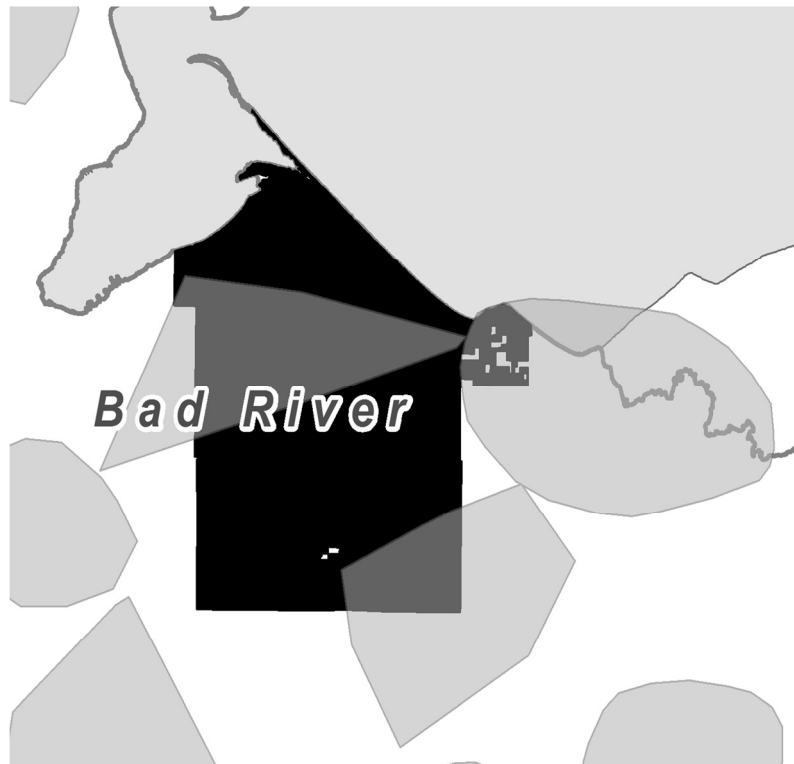
DIAGRAM 2—WOLF PACK TERRITORIES ON THE BAD RIVER RESERVATION 141
